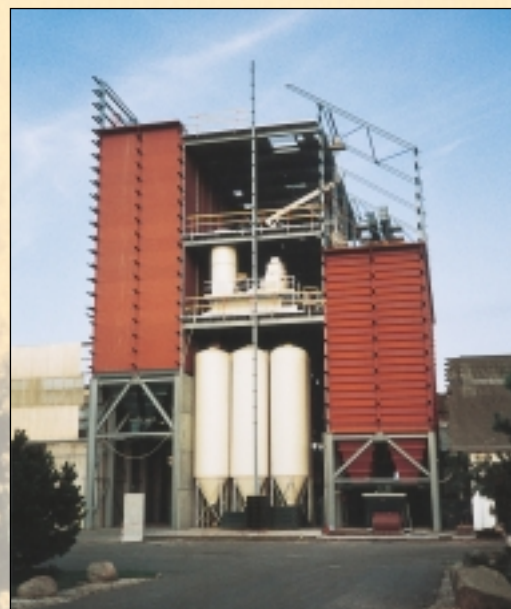
Silo for raw and mixed foodstuff for a feed mill with steel structure and machine deck
